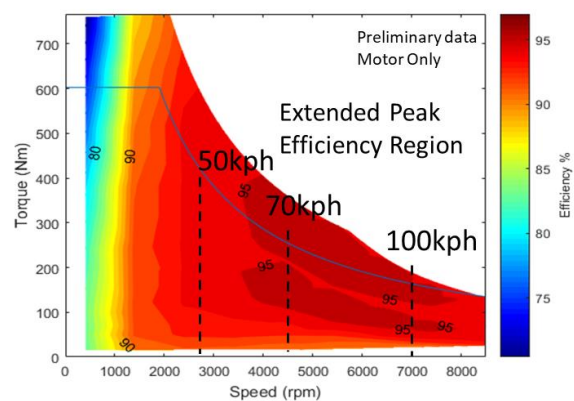
HDSRM300 Performance & Efficiency Curves
