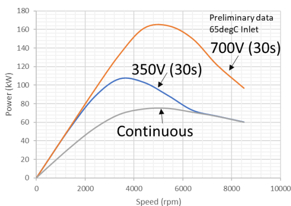
HDSRM300 Performance & Efficiency Curves
